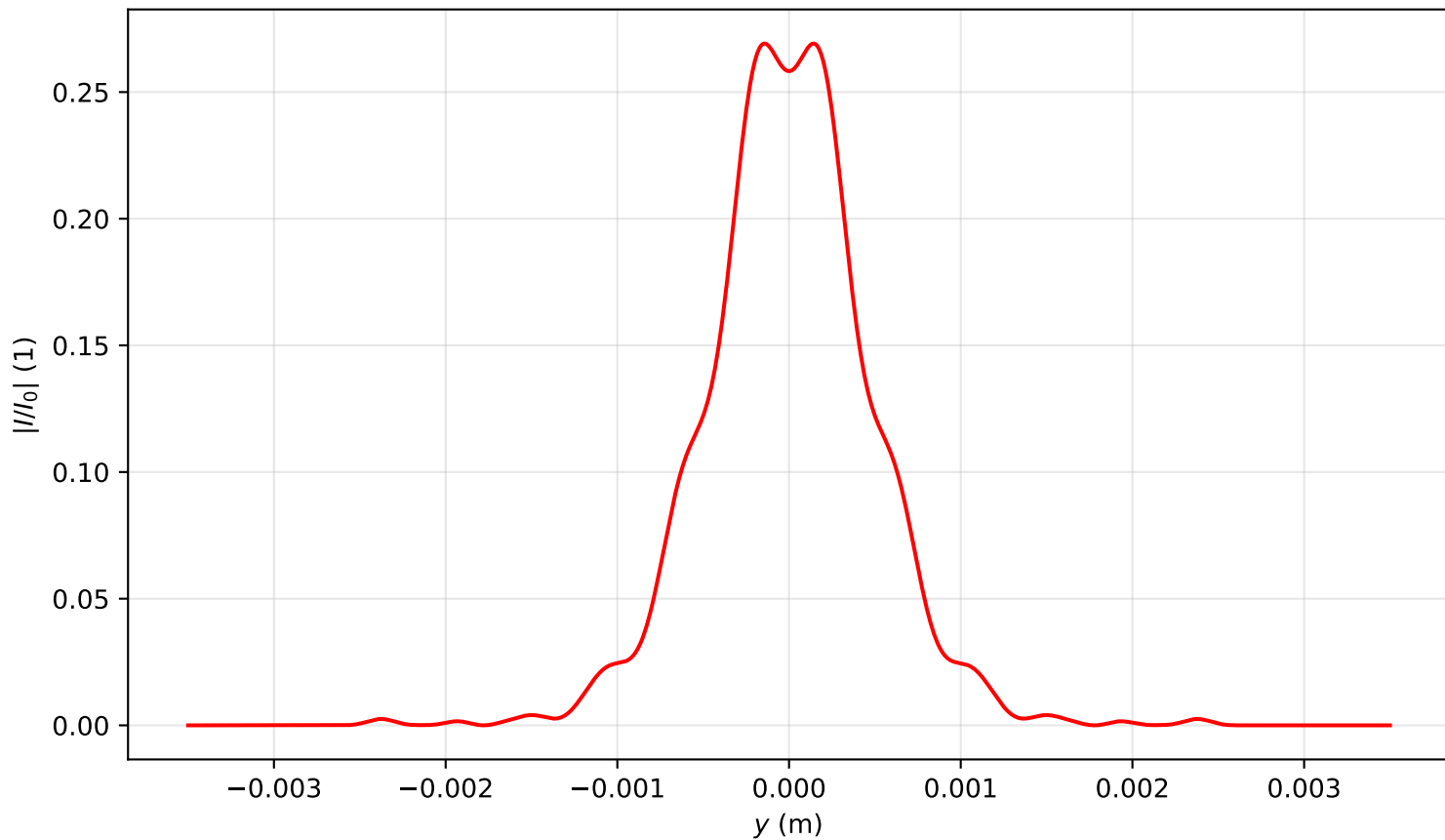
Intensity profile I(x=0, y, z=3.025)/I_0 , P_{in}=1.0P_{cr} , artificial time
